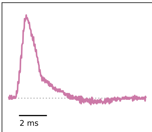
Mechanical pulse (rod displacement)
